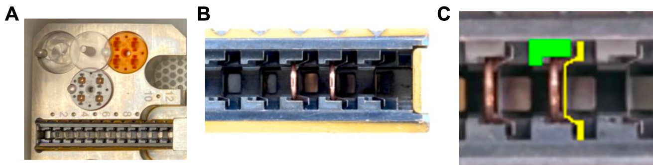
Figure 11. Correctly loaded autogrids. A) The grid box lid secures the autogrid boxes in the metal block. B&C) The grids sit between the L (highlighted green) and the spring (highlighted yellow).
