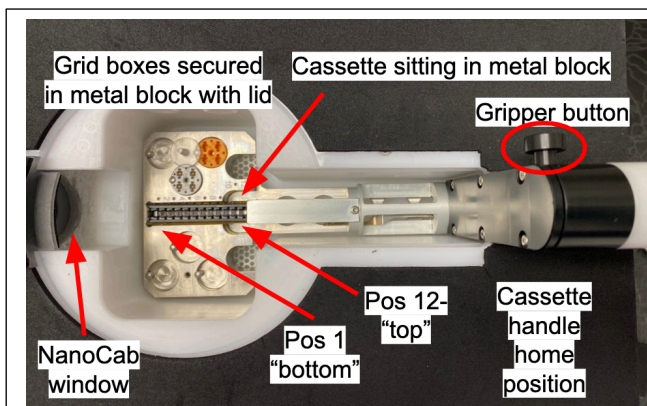
Figure 8. Assembled transfer station shown without covers or LN 2 for detail. Cassette is in loading position and gripper is secured in home position.
