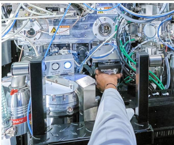
Figure 12. Highlight of Krios autoloader dock, with hand placing NanoCab for docking. Indicator lights and loading buttons are to the left.
