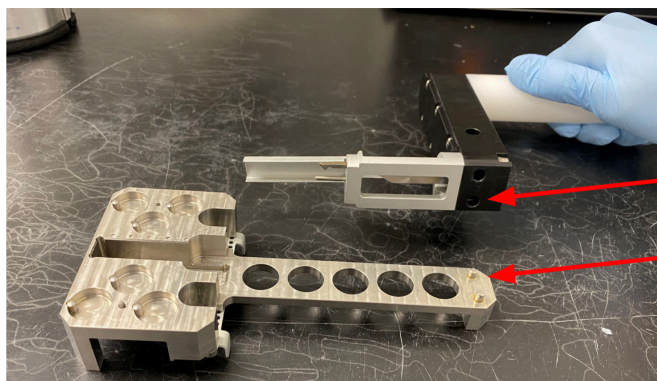
Figure 10. Metal block and gripper are shown outside the loading station at room temperature to highlight the holes in the gripper that position it in a stable “homed” position on the metal block.
